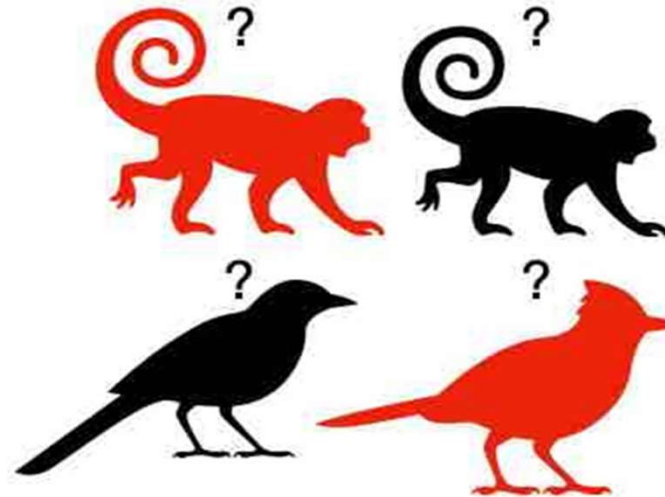
Unlabelled data
