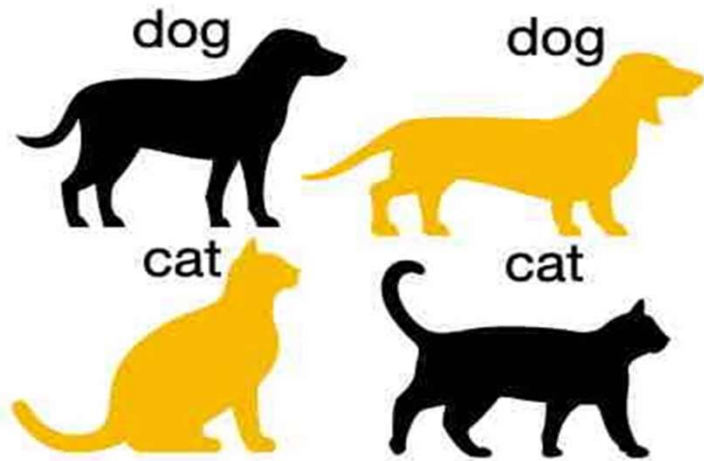
Labelled data
